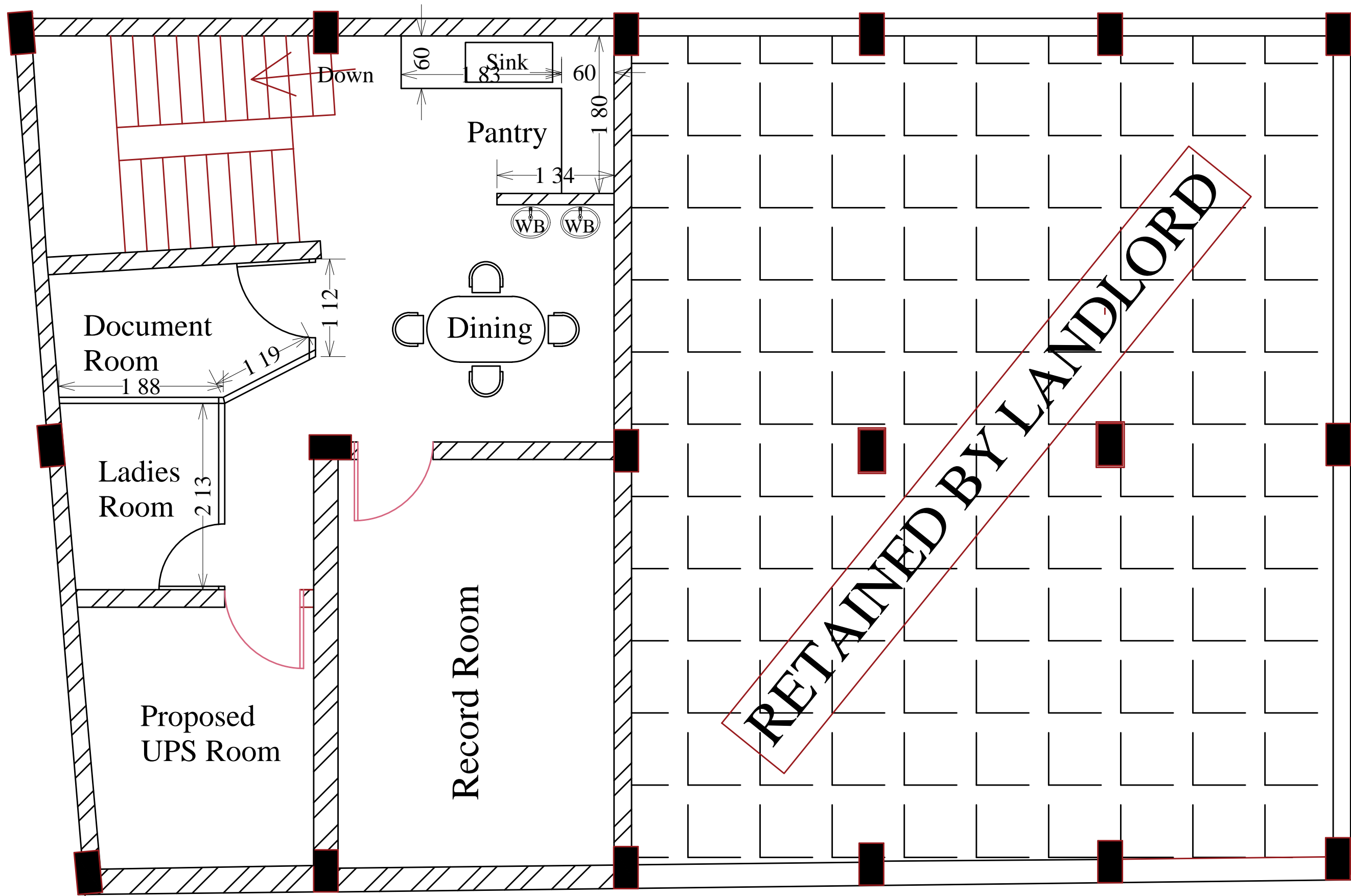
SBI CHERUTHURUTHY BRANCH - PROPOSED FF LAYOUT
